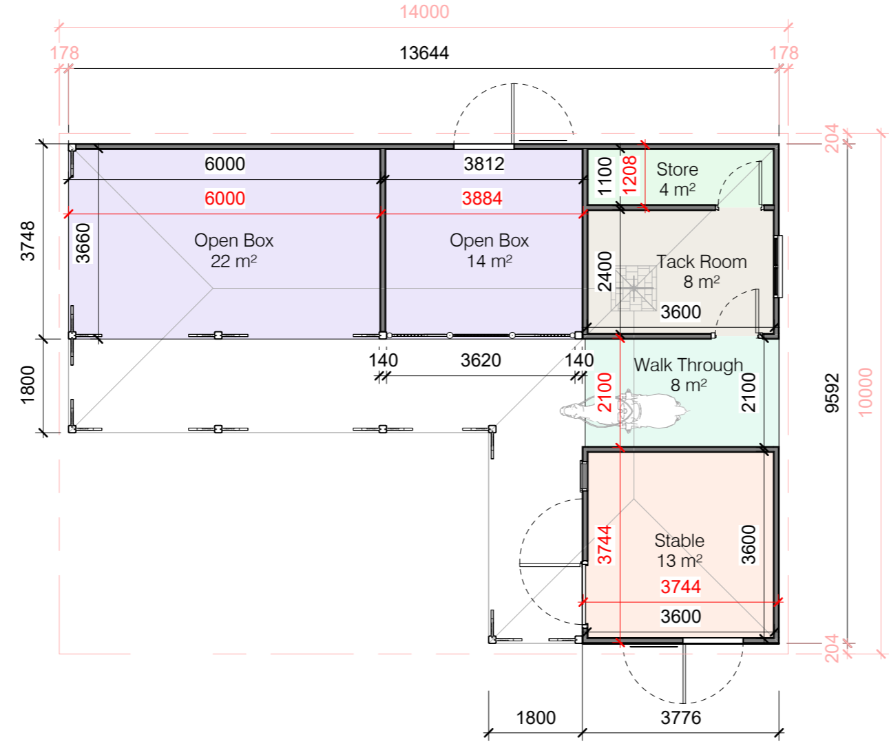
1 Proposed Layout PL- 4594 1 : 100
