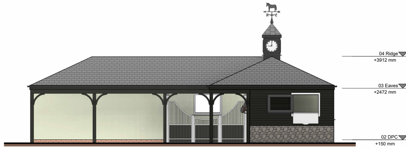
1 South Elevation E-4594 1 : 100
