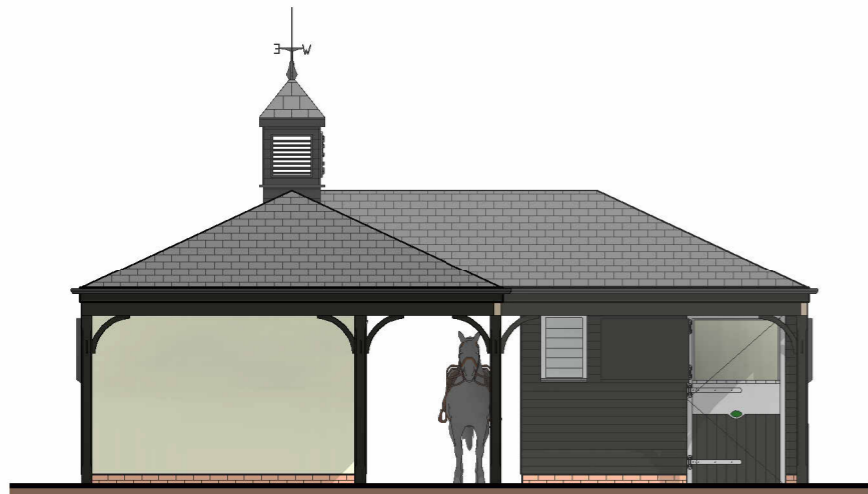
3 West Elevation E-4594 1 : 100
