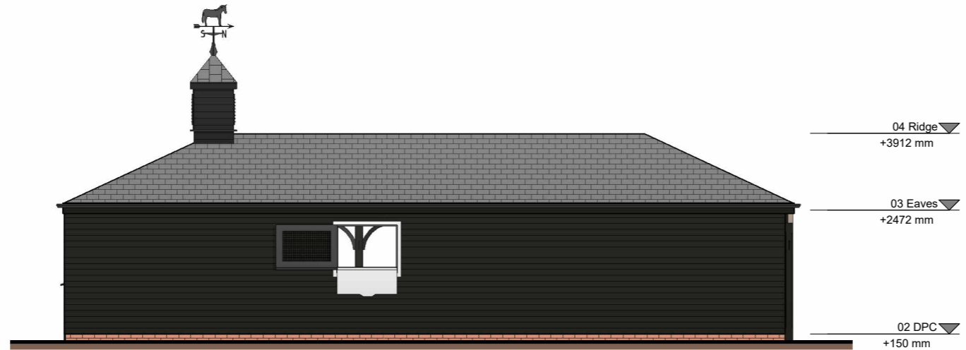
2 North Elevation E-4594 1 : 100
