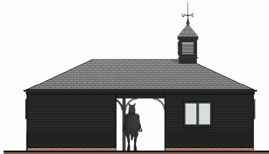
4 East Elevation E-4594 1 : 100
